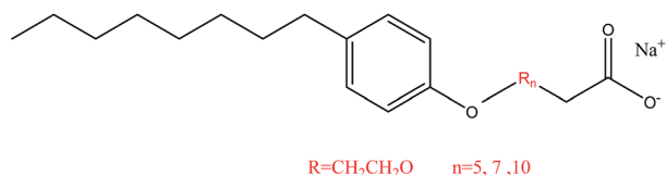
Scheme 1 The chemical structures of NPEC-5, NPEC-7, and NPEC-10.
