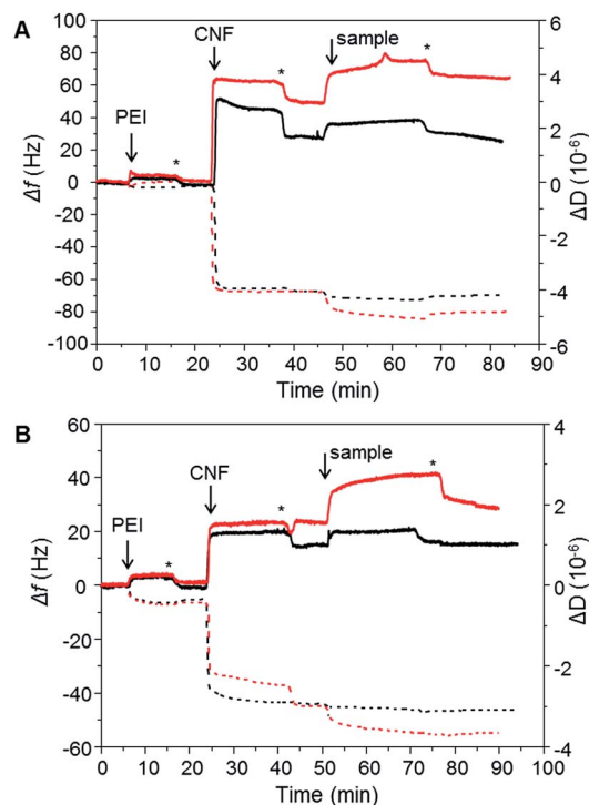
Fig. 4 In situ QCM-D experiment showing adsorption of PEI, CNF and the polymer samples. (A) PSBMA 266 (black lines) and XG-b-PSBMA 266 (red lines), (B) PSBMA 710 (black lines) and XG-b-PSBMA 710 (red lines). Change in frequency, \Delta f , (dashed lines) and change in dissipation, \Delta D , (solid lines). Rinsing steps with MilliQ water are denoted with an asterisk (*).
