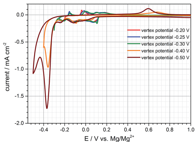
Fig. 2 Negative vertex potentials below -0.25 \text{ V} vs. \text{Mg}/\text{Mg}^{2+} worsen reversible electrochemical reactions of magnesium intercalation/deintercalation into/from graphite and lead to \text{Mg} -metal deposition and severe electrolyte decomposition in combination with shifted anodic peaks and huge overpotentials respectively.
