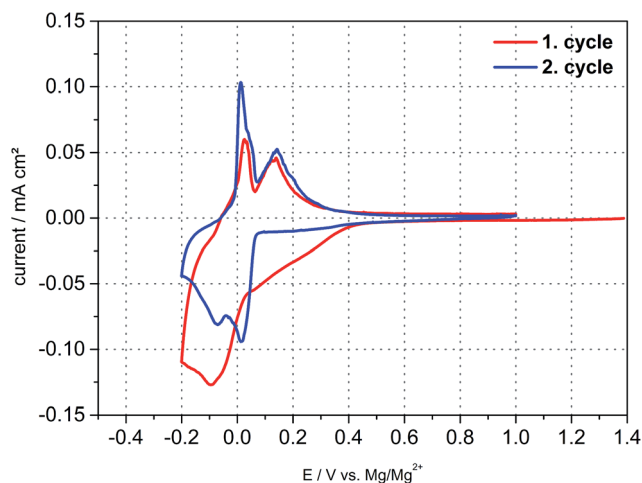
Fig. 5 Cyclic voltammogram of a natural graphite electrode vs. magnesium metal in 0.1 M \text{TBA-BF}_4/\text{DMF} at a scan rate of 0.05 \text{mV s}^{-1} . The intercalation and deintercalation of \text{TBA}^+ -ions into and from graphite resembles the intercalation behaviour of magnesium into graphite.
