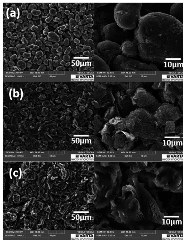
Fig. 3 (a) SEM images of a pristine graphite anode showing the potatoo shaped graphite particles. (b) SEM images of a cycled graphite anode in 0.5 \text{ M Mg}(\text{TFSI})_2/\text{DMF} revealing a homogeneous electrode surface after many electrochemical cycles. (c) SEM images of the graphite surface after polarizing the electrode below -0.3 \text{ V} vs. \text{Mg}/\text{Mg}^{2+} and to deeper voltages leading to passivation and exfoliation of the graphite particles.
