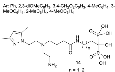
Scheme 2 Reagents and conditions: (i) H 3 PO 3 , PCl 3 . (ii) ArCOCl, NaOH.
