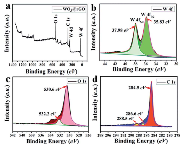
Fig. 4 XPS spectra of as-obtained \text{WO}_3 -rGO composite: (a) survey scan; high-resolution (b) W 4f, (c) O 1s, and (d) C 1s spectrum.
