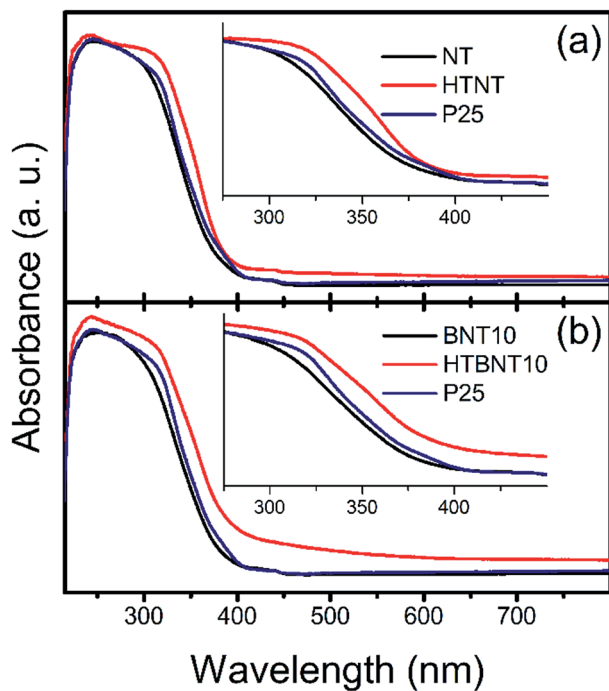
Fig. 7 UV-VIS absorption spectra of the pristine titanate nanotubes (a), and nanotubes decorated with 10% BiOCl (b) before (NT and BNT10) and after (HTNT and HTBNT10) annealing. Results for Degussa P25 are also shown for comparison.
