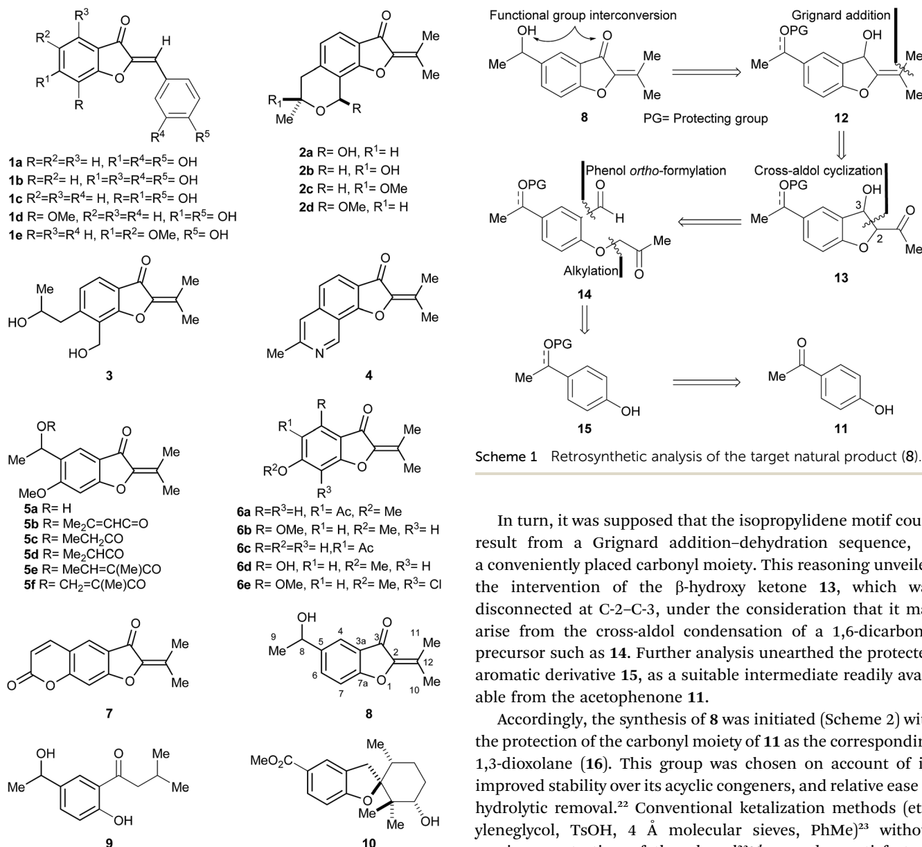
Fig. 1 Natural products carrying the 2-isopropylidene benzofuran-3-one motif, and related structures.
