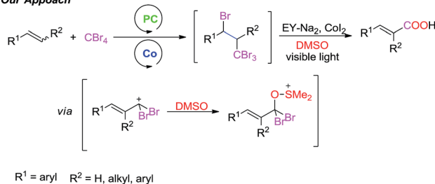
Scheme 1 Carboxylation of styrenes.
