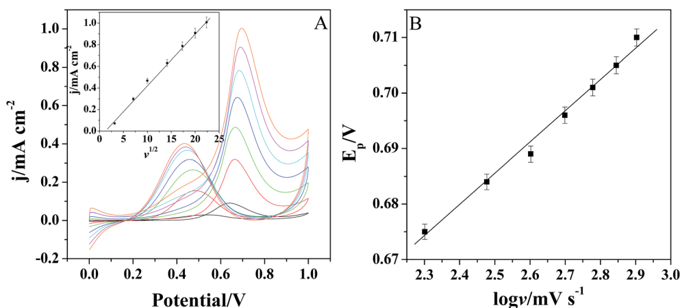
Fig. 6 (A) The CVs of Pt/[(PDDA-GS) 3 /(PEDOT:PSS) 2 ]/GCE to methanol oxidation at different scan rates (from bottom: 10, 50, 100, 200, 300, 400, 500 \text{mV s}^{-1} ). Inset: the relationship of I_f vs. the square root of scan rate. (B) The relationship between peak potential E_p of methanol oxidation and \log v . The error bars show the standard deviations taken from three tests.
