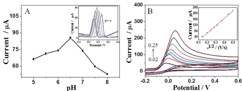
Fig. 5 (A) Effect of pH value on the oxidation current response of 2.5 mM AA at NCN/GCE. Inset: DPVs of 2.5 mM AA at NCN/GCE with different pH values (a → g: 5, 5.5, 6, 6.5, 7, 7.5, 8); (B) CVs of 5 mM AA in 0.1 M PBS (pH 6.5) at NCN/GCE with different scan rates (0.02, 0.04, 0.06, 0.08, 0.10, 0.14, 0.2 and 0.25 V s -1 ). Inset: the oxidation peak current of AA vs. the square root of the scan rate.
