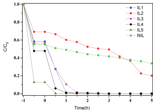
Fig. 6 Photocatalytic activities for degradation of RhB dye under visible-light irradiation in the presence of \text{SnS}_2 samples.
