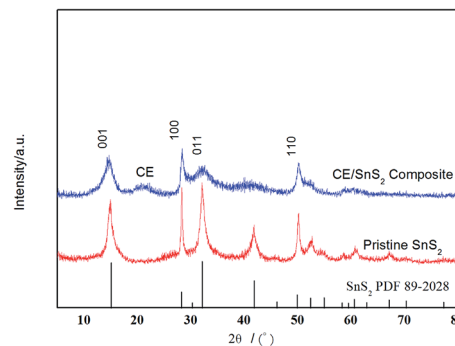
Fig. 7 XRD pattern of pristine \text{SnS}_2 (IL4) and \text{CE}/\text{SnS}_2 composite.
