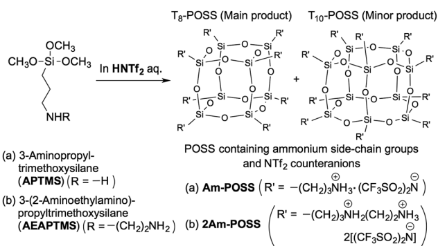
Scheme 2 Preparation of POSSs containing ammonium side-chain groups and \text{NTf}_2 counteranions: (a) Am-POSS and (b) 2Am-POSS .
