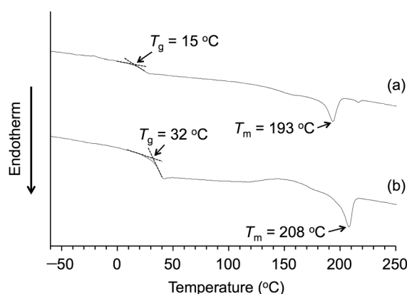
Fig. 13 DSC curves of (a) Am-POSS and (b) 2Am-POSS under a nitrogen flow.
