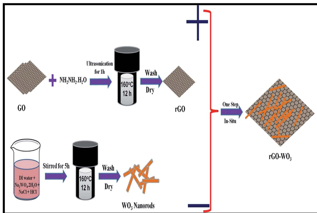
Fig. 1 Schematic of synthesis steps used for the synthesis of WO 3 NRs and rGO–WO 3 composite.
