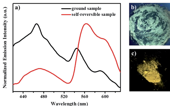
Fig. 6 (a) PL spectra of complex 1 at different conditions. Excitation wavelength: 365 nm. Photographic images of luminogen 1 under 365 nm UV light: (b) the entirely ground sample; (c) 10 h after grinding.
