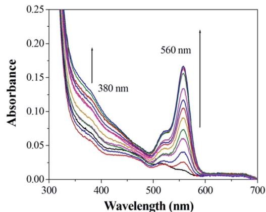
Fig. 6 The absorption change profile of sensor 1 (1 \mu\text{M} ) to different metal ions (2 mM) in 0.1 M Tris-HCl solution (ethanol-water = 1 : 10, v/v, pH 7.14).
