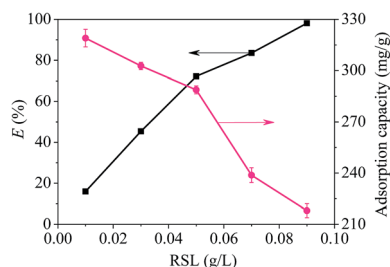
Fig. 9 Effects of adsorbent dosage on the removal of mercury(II). Condition: T = 300 K, C_0 = 20 mg L -1 , pH = 7.0 ± 0.1.
