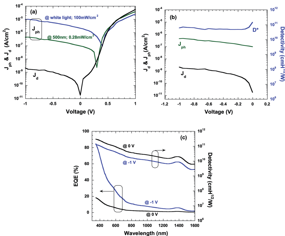
Fig. 4 (a) Current–voltage ( J – V ) characteristics of polymer photodetectors measured in the dark and under illumination with \lambda = 500 nm and white light; (b) photocurrent, dark current, and estimated detectivities at \lambda = 500 nm vs. biased voltages; and (c) EQE vs. wavelength and estimated detectivities vs. wavelength at the biases of 0 V and -1 V.
