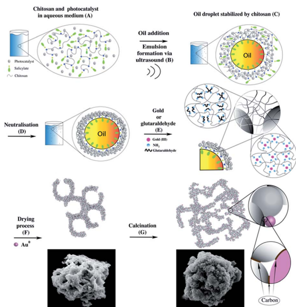
Fig. 6 Microparticles formation mechanism: TiO 2 dispersion in chitosan solution (A), oil droplets stabilized by chitosan (C), neutralisation (D), gold or glutaraldehyde addition and effects (E), drying (F) and calcination (G).
