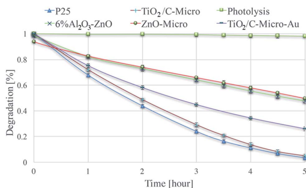
Fig. 7 Degradation of metanil yellow via photolysis and via photo-degradation with P25, TiO 2 /C-Micro, TiO 2 /C-Micro-Au, 6% Al 2 O 3 -ZnO and ZnO-Micro.
