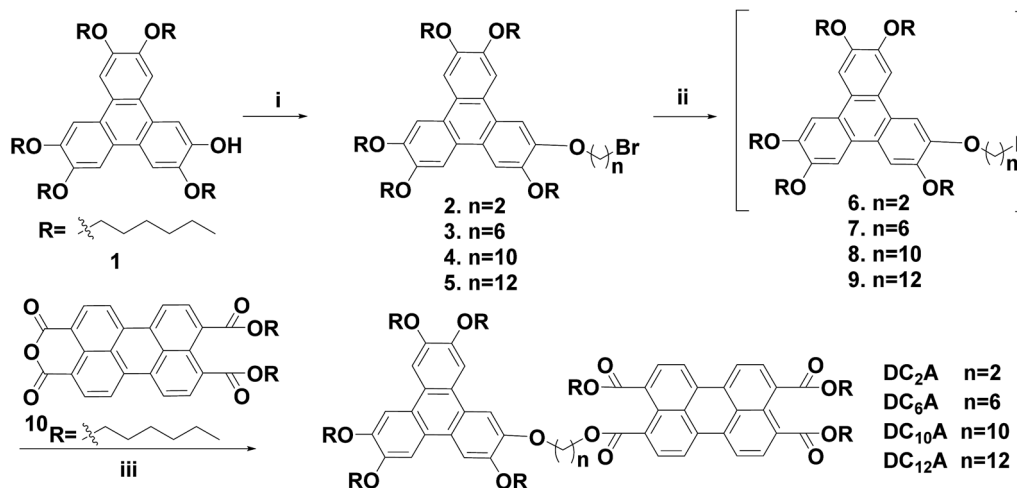
Scheme 1 Synthesis of D–A dyads based on triphenylene and perylene cores. Reagents and conditions: (i) \text{KOH} , \text{H}_2\text{O} , 1 , \omega -dibromoalkanes, tetrabutylammonium bromide, dichloromethane, rt, 24 h, 68–93%; (ii) \text{KI} , acetone, refluxing, 24 h; (iii) \text{K}_2\text{CO}_3 , 1-hexanol, 50 °C, 72 h, 28–40% (two steps).
