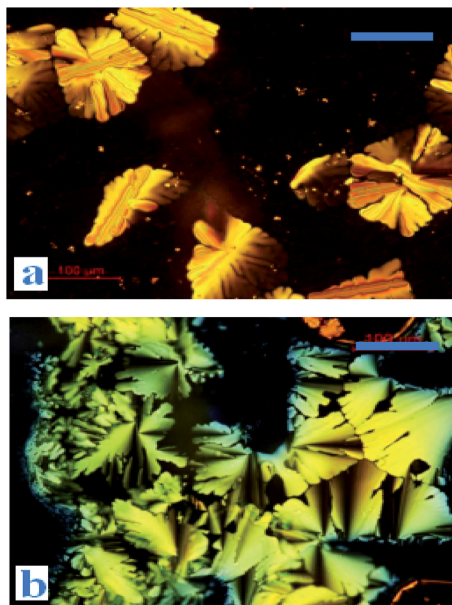
Fig. 2 Optical textures of \text{DC}_{10}\text{A} at 68 °C (a) and \text{DC}_{12}\text{A} at 48 °C (b) on cooling from the isotropic liquid, crossed polarizers, scale bar 100 \mu\text{m} .
