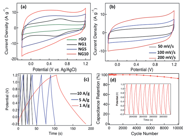
Fig. 3 (a) Cyclic voltammograms of rGO, NG1, NG5 and NG10 using a three-electrode cell at a scan rate of 100 mV s -1 in 0.5 M H 2 SO 4 solution, (b) cyclic voltammograms of NG10 at different scan rates (50, 100 and 200 mV s -1 ) in a two-electrode T-cell system, (c) galvanostatic charge/discharge curves for NG10 in a two-electrode T-cell system tested at current density of 1–10 A g -1 , (d) cycling stability of NG10 measured at 5 A g -1 over the potential range of 1.2 to -0.2 V. The inset shows the charge–discharge curves over the last ten cycles.
