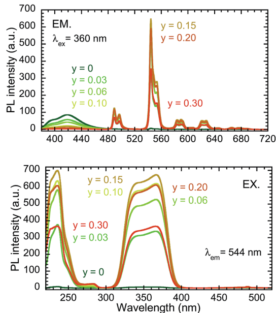
Fig. 3 PL and PLE spectra of samples from the Y_{0.98-y}Ce_{0.02}Tb_yBO_3 library ( 0 \leq y \leq 0.3 ).
