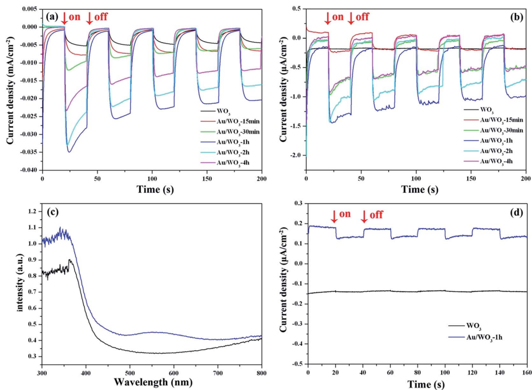
Fig. 6 Photocurrent response of \text{WO}_3 and \text{Au}/\text{WO}_3\text{-X} samples (a) under simulated sunlight irradiation, and (b) under visible light ( \lambda > 420 \text{ nm} ) irradiation. (c) UV-Vis diffuse reflectance spectra, and (d) photocurrent response with \lambda > 520 \text{ nm} light irradiation of the bare \text{WO}_3 and \text{Au}/\text{WO}_3\text{-1 h} samples.
