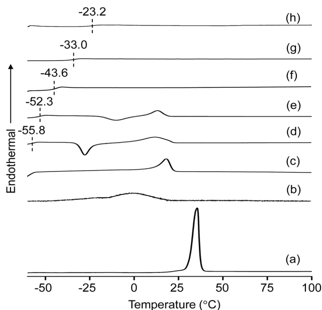
Fig. 1 DSC thermograms of: (a) ED2003, (b) M-2070 and MP(70 : 30)-Z blended hybrid SPEs with Z = (c) ∞, (d) 32, (e) 24, (f) 16, (g) 12 and (h) 8. Z indicates the [O]/[Li] ratio.
