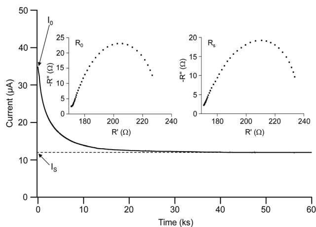
Fig. 5 Typical depolarization curve of the MP(70 : 30)-16 blended hybrid SPE.
