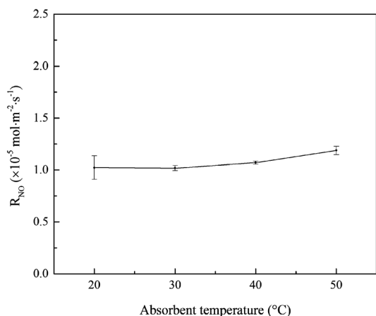
Fig. 6 Effects of absorbent temperature on NO absorption rate (conditions: active chlorine concentration, 1500 mg L ^{-1} [Cl _2 ]; NO inlet concentration, 1000 ppm; SO _2 inlet concentration, 0 ppm; solution pH, 7).
