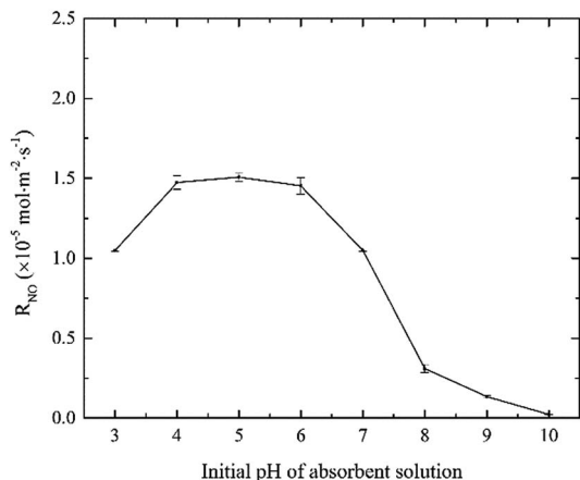
Fig. 5 Effects of solution pH value on NO absorption rate (conditions: active chlorine concentration, 1500 mg L ^{-1} [Cl _2 ]; NO inlet concentration, 1000 ppm; SO _2 inlet concentration, 0 ppm; absorbent temperature, 20 °C).
