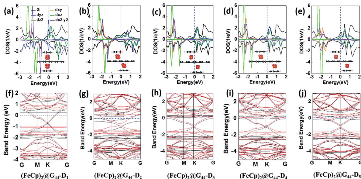
Fig. 5 (a–e) Density of states (DOS) and (f–j) band structure plots of (FeCp) 2 @G 44 s. Insets are the spin densities plots.
