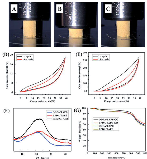
Fig. 5 Compressible properties of ODA-TAPB PI aerogel (A–C), and stress–strain curves of (D) ODA based PI aerogel and (E) PI/GO nanohybrid aerogel for the first (black) and tenth (red) test cycles. And (F) PXRD patterns and (G) TGA curves of the PI aerogels and PI/GO nanohybrid aerogels.
