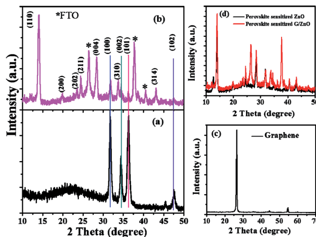
Fig. 2 XRD patterns of (a) spray deposited ZnO film on a glass substrate, (b) perovskite film on a ZnO/FTO-coated glass substrate, (c) graphene and (d) perovskite sensitized ZnO and G/ZnO nanocomposite films.
