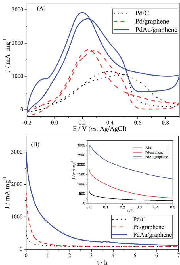
Fig. 5 (A, B) CV and CA results of HCOOH on PdAu/graphene, Pd/graphene and Pd/C catalysts ( 50\ mV\ s^{-1} ) for formic acid electro-oxidation in 0.5\ M\ H_2SO_4/0.5\ M\ HCOOH solutions. CA curves were recorded at 0.2\ V .
