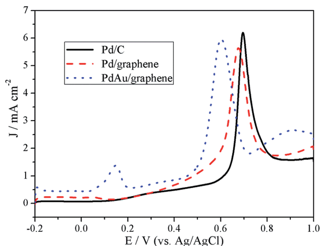
Fig. 7 CO stripping curves of the Pd/C, PdAu/graphene and Pd/graphene catalysts in 0.5\ M\ H_2SO_4 .
