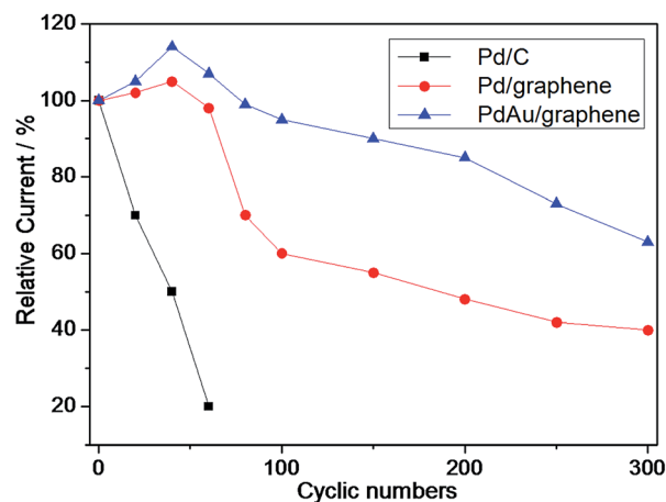
Fig. 6 Durability of PdAu/graphene and Pd/C electrocatalysts for formic acid electro-oxidation in 0.5\ M\ H_2SO_4 + 0.5\ M\ HCOOH solutions.
