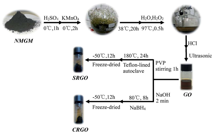
Fig. 1 The preparation process of GNs using NMGMs as the raw material.
