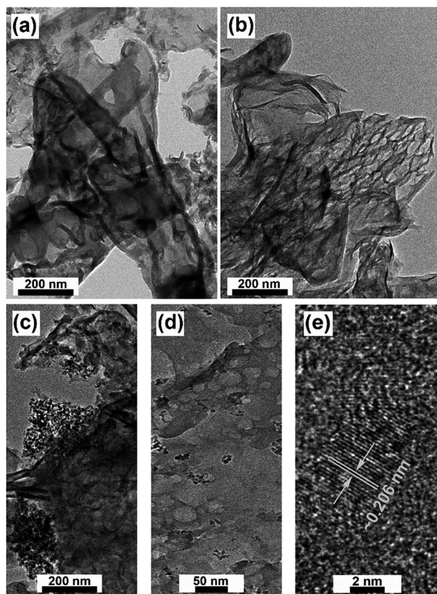
Fig. 2 TEM images of (a) g-C 3 N 4 , (b) large scale g-C 3 N 4 -DND (0.4 wt%), (c) g-C 3 N 4 -DND (40 wt%), (d) small scale g-C 3 N 4 -DND (0.4 wt%), and (e) HRTEM image of g-C 3 N 4 -DND (0.4 wt%).
