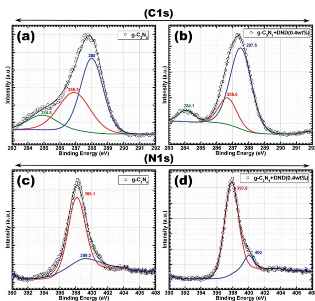
Fig. 3 XPS C 1s spectra of (a) g-C 3 N 4 and (b) g-C 3 N 4 -DND (0.4 wt%); N 1s spectra of (c) g-C 3 N 4 and (d) g-C 3 N 4 -DND (0.4 wt%).
