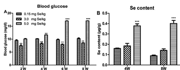
Fig. 1 Effects of supranutritional Se status on the level of blood glucose and Se content of pancreas ( \mu g g -1 wet weight). Chicks were fed the basal diet with 0.15 mg kg -1 Se (C-Se), 3.0 mg kg -1 Se (S-Se), and 5.0 mg kg -1 Se (E-Se). Effects of dietary Se concentration on blood glucose test in chicken on 2 nd , 4 th , 6 th , and 8 th week. Values are means \pm S.D., n = 6 . * P < 0.05 ; ** P < 0.01 , *** P < 0.001 compared with the C-Se group (A). Pancreatic Se contents in chicken on 4 th and 8 th week. * P < 0.05 , ** P < 0.01 , *** P < 0.001 compared with the C-Se group (B).
