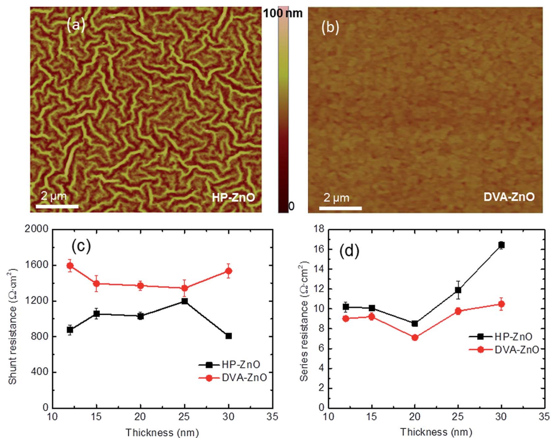
Fig. 3 AFM images of ZnO films with the following annealing method: (a) 200 ^{\circ} C hot plate annealing for 60 min. (b) 200 ^{\circ} C vacuum oven annealing for 90 min. (c) Shunt resistance–thickness characteristic of IPSCs. (d) Series resistance–thickness characteristic of IPSCs.
