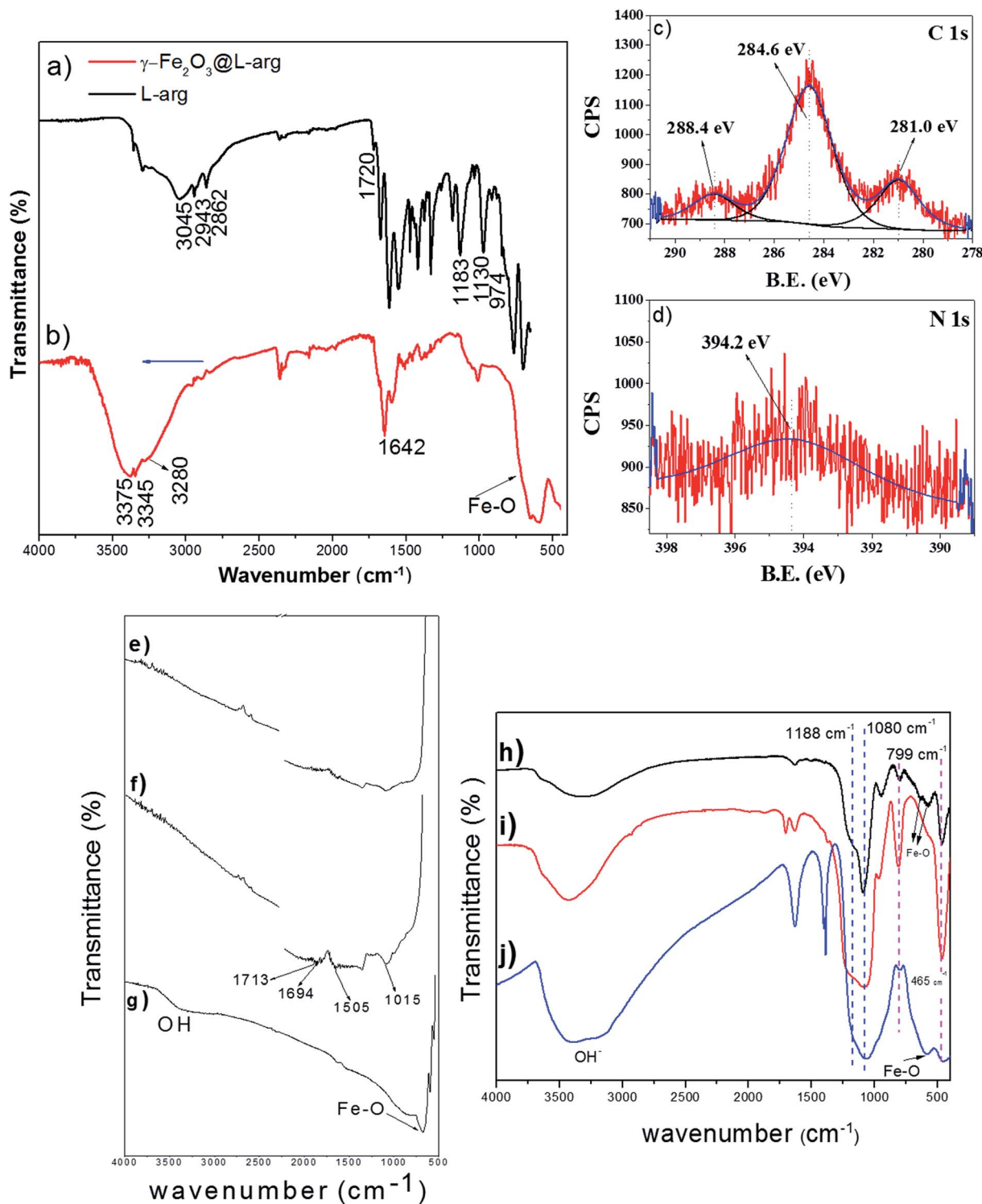
Fig. 3 FTIR of pure L-arg (a), \gamma\text{-Fe}_2\text{O}_3\text{@L-arg} (b), C 1s and N 1s XPS regions for \gamma\text{-Fe}_2\text{O}_3\text{@L-arg} Nps (c and d), MWCNTs, FTIR signal in the range 2700–400 \text{cm}^{-1} is 5 \times enhanced (e), o-MWCNTs, FTIR signal in the range 2700–400 \text{cm}^{-1} is 5 \times enhanced (f), \gamma\text{-Fe}_2\text{O}_3\text{@MWCNTs} (g), \gamma\text{-Fe}_2\text{O}_3\text{@SiO}_2 Nps (h), pure SBA15 (i) and \gamma\text{-Fe}_2\text{O}_3\text{-SBA15} (j).
