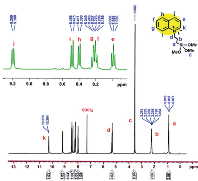
Fig. 1 1 H NMR spectrum of TMSQI.
