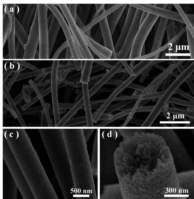
Fig. 1 (a) A typical SEM image of the as-spun polymer precursor for sample A. (b–d) Typical SEM images of the obtained loaded sample A under different magnifications.
