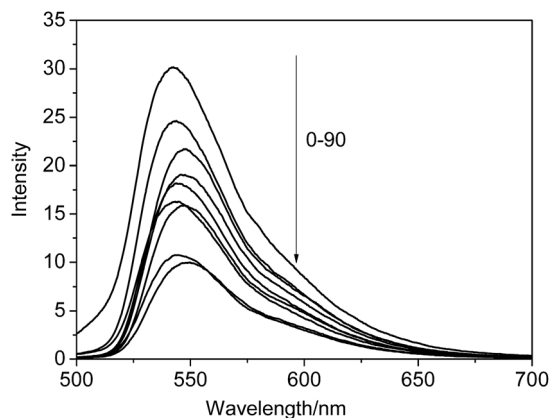
Fig. 2 Temperature dependent fluorescent changes of NP/Cu(OAc) 2 metallogel. Unit for 0–90: °C.
