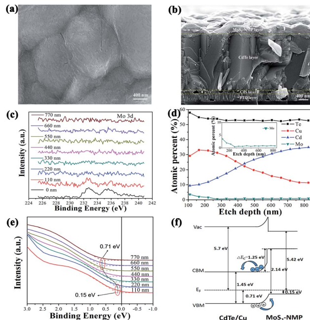
Fig. 4 (a) High magnification SEM image of CdTe surface after spin-coating three times. (b) The cross-sectional view of the best CdTe cell (3T- \text{MoS}_2 ). (c) The XPS spectra of Mo element with etching depth in CdTe cell (3T- \text{MoS}_2 ). (d) The atomic percent of Cd, Te, Cu and Mo with etching depth for CdTe cell (3T- \text{MoS}_2 ). (e) The valence spectra of CdTe cell (3T- \text{MoS}_2 ) with etching depth. (f) The energy band structure of CdTe solar cells (3T- \text{MoS}_2 ).
