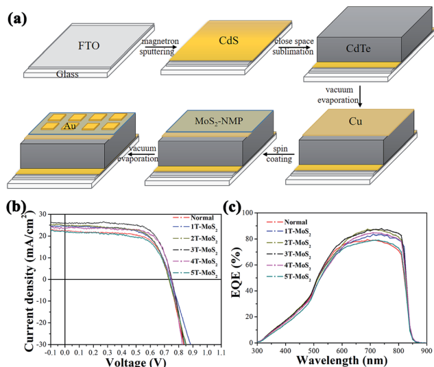
Fig. 3 (a) Fabrication procedure of CdTe solar cells. (b) Current density–voltage ( J – V ) curves of solar cells after spin-coating \text{MoS}_2 –NMP solution zero, once, twice, three, four and five times under AM 1.5 illumination. (c) The EQE spectra of corresponding six solar cells.
