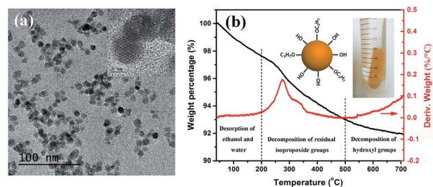
Fig. 1 (a) TEM image (inset: HR-TEM image of the nanoparticles), and (b) TG-DTG curves of the \text{BaTiO}_3 nanoparticles. The inserted photograph is the as-prepared “gel rod” in ethanol: a collected rod composed of fully crystallized nanoparticles as observed in (a).
