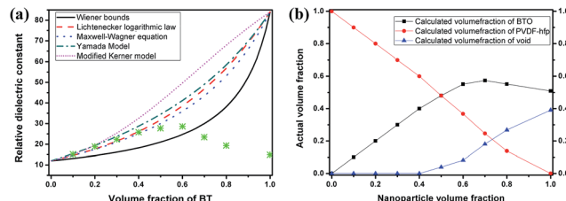
Fig. 6 (a) Experimental and theoretical predicted relative dielectric constant of the nanocomposite films at different BT volume fractions at 1 kHz. (b) The calculated volume fractions of BT, PVDF–hfp and voids in the nanocomposite films in terms of the designed BT volume fractions by Lichtenecker logarithmic law.
