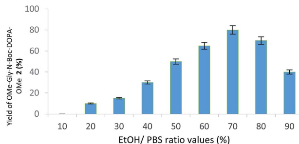
Fig. 1 Yield (%) of OMe-Gly-N-Boc-DOPA-OMe 2 during the oxidation of BTO 1 with tyrosinase from Agaricus bisporus in the presence of NH 2 -Gly-OMe at different EtOH/PBS ratio values. Experiments were conducted on triplicate.
