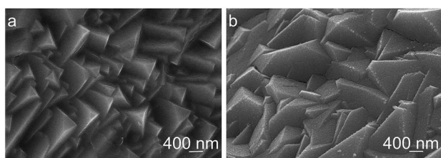
Fig. 12 Morphology of \text{Cu}_2\text{O} foam electrodes surface during photoelectrocatalytic reaction. (a) Before reaction, (b) after reaction for 1.5 h.
