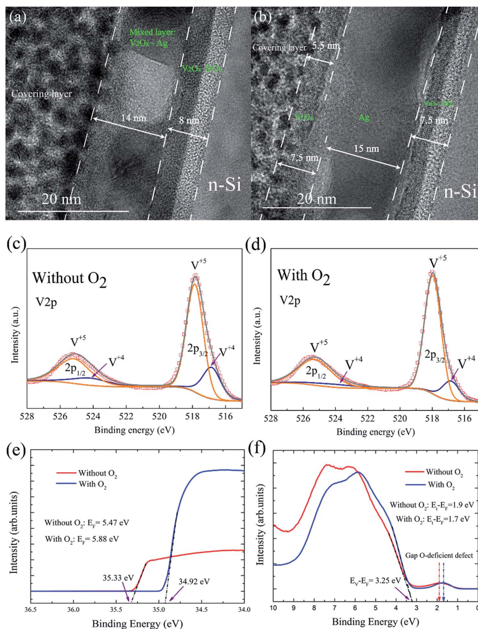
Fig. 2 Cross-sectional TEM micrographs of \text{V}_2\text{O}_x (8 nm)/Ag ( x nm)/ \text{V}_2\text{O}_x (8 nm) multilayer films with (a) x = 4 \text{ nm} Ag and (b) x = 16 \text{ nm} Ag. (c) and (d) XPS spectra of \text{V}_2\text{O}_x films prepared without and with the introduction of an \text{O}_2 partial pressure into the thermal evaporation process, respectively. The UPS spectra of \text{V}_2\text{O}_x films: (e) the work function ( E_F ); (f) shows the positions of the O-deficiency in-gap defect states near the Fermi level.
