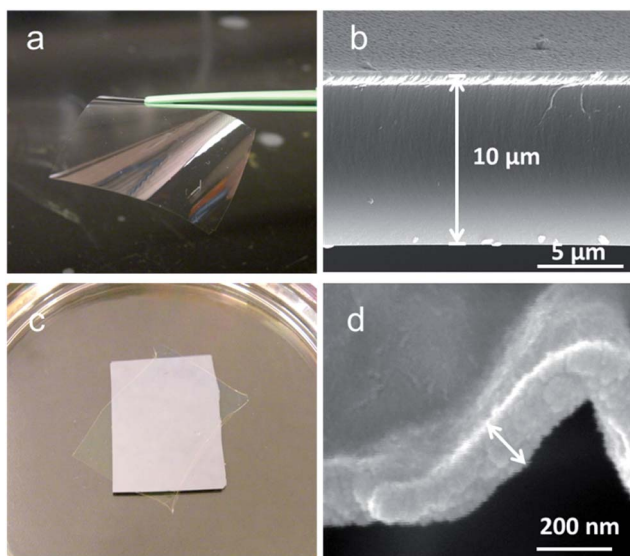
Fig. 2 Optical and SEM images of the fabricated Janus films with thickness of 10 \mu\text{m} (a) and (b), and 150 nm (c) and (d).
