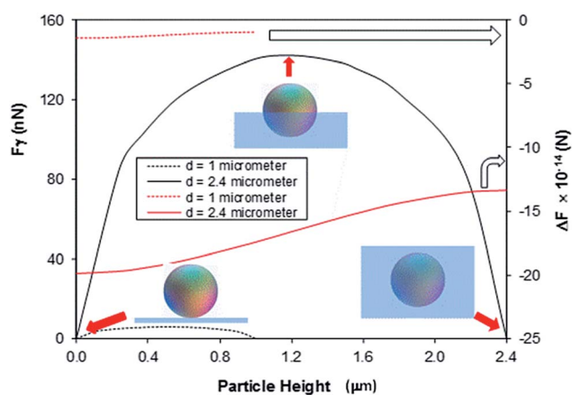
Fig. 9 Surface tension force ( F_{\gamma} ) and the difference between weight and the buoyancy forces ( \Delta F = W - F_B , where W is the weight of spherical particle and F_B is the buoyancy force) with the height of immersed spherical dust particles. For particle diameter of 2.4 \mu\text{m} , h = 0 represents dust particles on silicon oil surface, h = 1.2 \mu\text{m} corresponds to the halfway immersed particle, and h = 2.4 \mu\text{m} corresponds to totally immersed particle.
