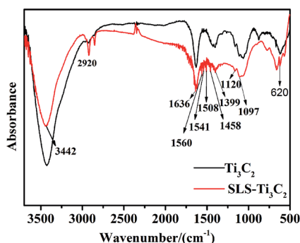
Fig. 3 FTIR spectra of \text{Ti}_3\text{C}_2\text{T}_x MXenes with and without surface functionalization.
