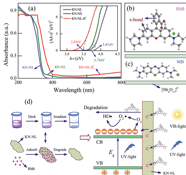
Fig. 6 (a) UV-VIS DRS of KN-NL, KN-NS and KN-NL-H + with the inset curve of (Ah\nu)^2 vs. h\nu . The molecular structure of (b) RhB and (c) MB. (d) The relevant kinetics mechanisms of adsorption and photocatalysis for KN-NL in RhB solution.
