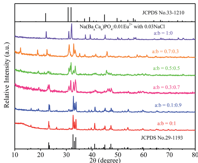
Fig. 5 XRD patterns of Na(Ba a Ca b )PO 4 :0.01Eu 2+ with 0.03NaCl and standard data (JCPDS no. 29-1193 and JCPDS no. 33-1210).
