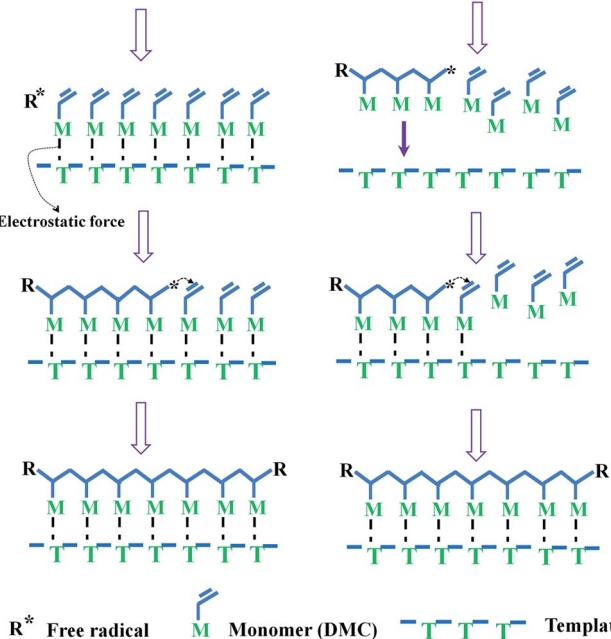
Fig. 2 The mechanism of template copolymerization.
