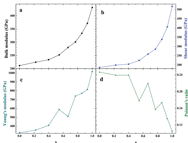
Fig. 4 Mechanical properties of \beta -Si 1-x C; bulk modulus (a), shear modulus (b), Young's modulus (c) and Poisson's ratio (d).
