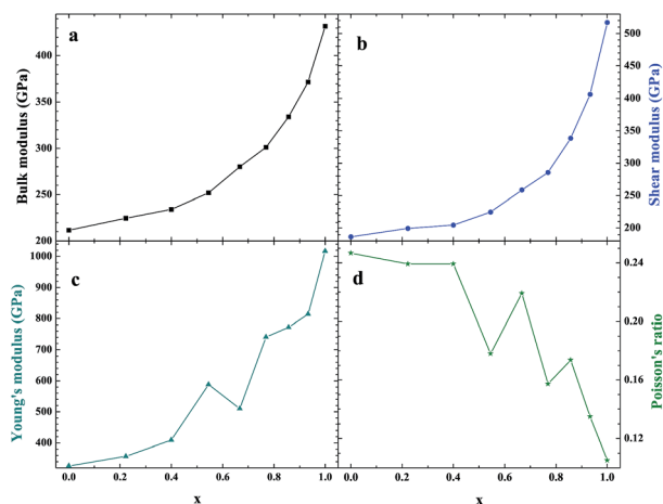
Fig. 4 Mechanical properties of \beta\text{-Si}_{1-x}\text{C} ; bulk modulus (a), shear modulus (b), Young's modulus (c) and Poisson's ratio (d).
