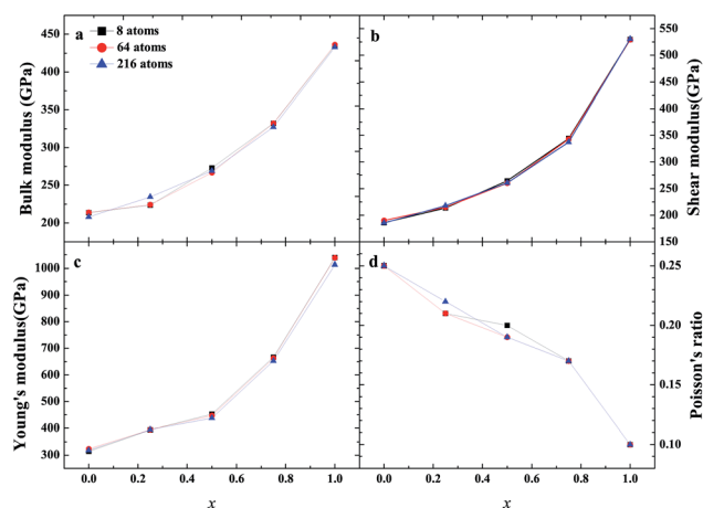
Fig. 5 Mechanical properties of \beta -Si 1-x C based on different supercell sizes; bulk modulus (a), shear modulus (b), Young's modulus (c) and Poisson's ratio (d).
