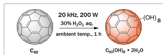
Fig. 2 Synthesis of water soluble fullerene via acoustic cavitation induced by ultrasound at ambient temperature, within 1 h reaction time and in the presence of dil. H_2O_2 (30%).
