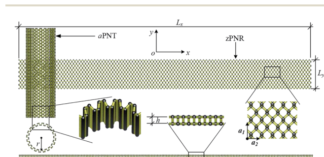
Fig. 1 Computational model of zPNR and aPNT. L_x , L_y and h are length, width and thickness of zPNR, respectively, and r is an in-between radius of aPNT. Lattice vectors \mathbf{a}_1 and \mathbf{a}_2 are along armchair( n,0 ) and zigzag( 0,m ) directions, respectively.
